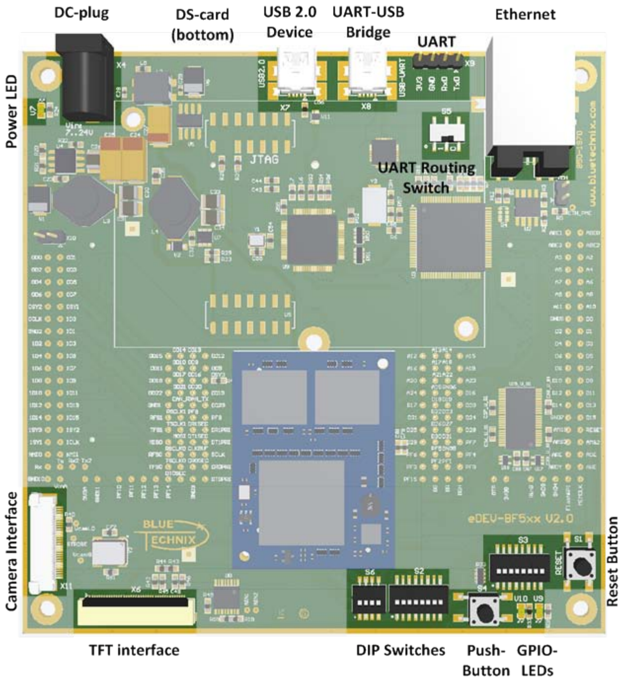
Figure 2-2: Interface overview
