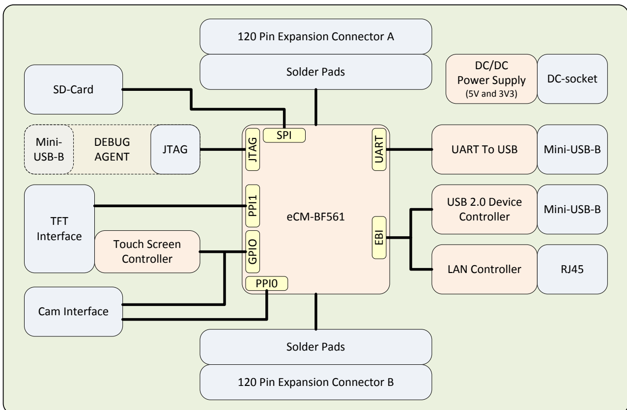
Figure 2-1: Interconnection diagram
