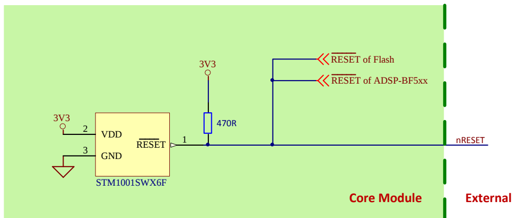
Figure 5-1: Reset circuit
