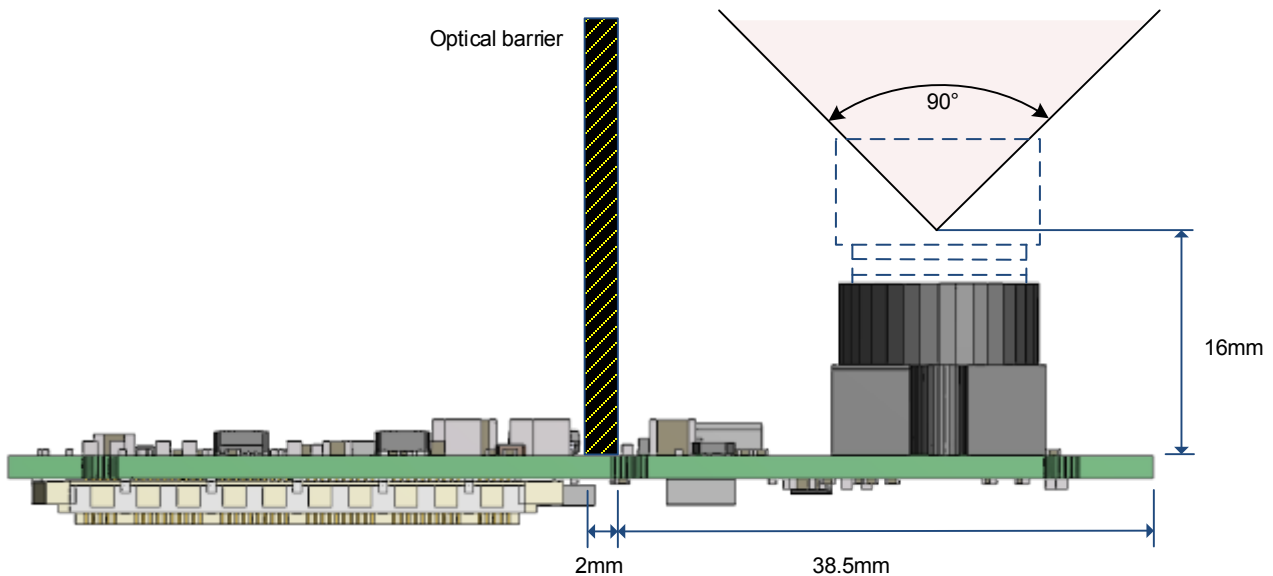
Figure 3-3: Optical isolation
