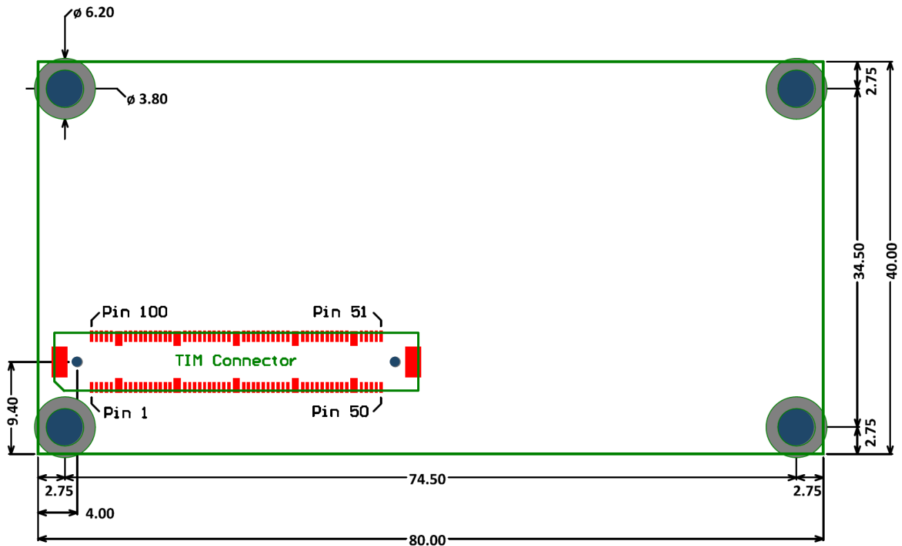
Figure 7-4 Footprint of the TIM UP – 19k-S3-Spartan6
