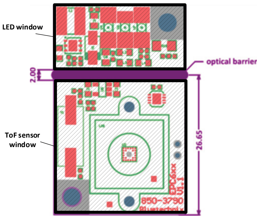
Figure 4-2: Mechanical dimensions for an optical barrier
