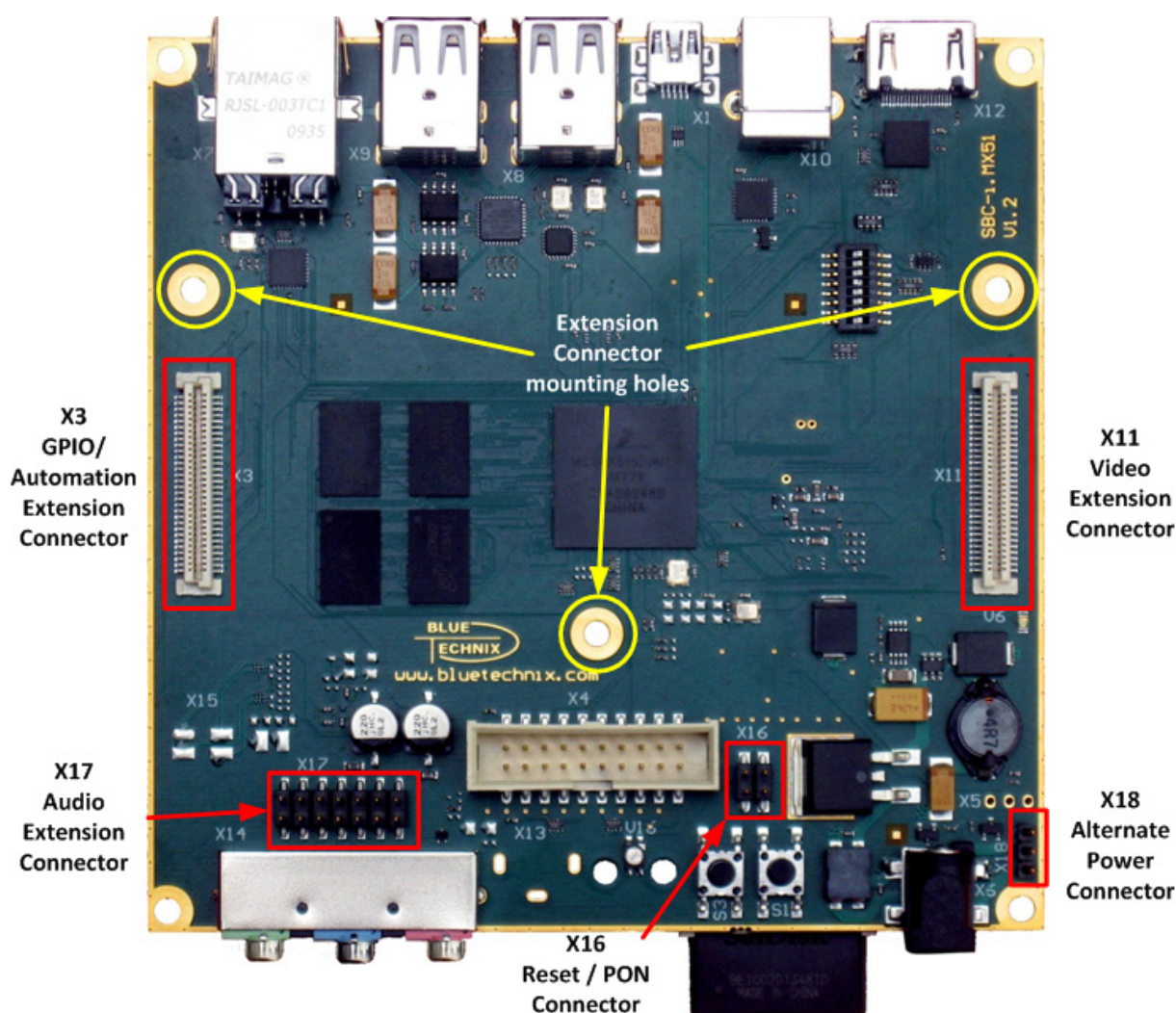
Figure 4-1: Extension Connector positions
