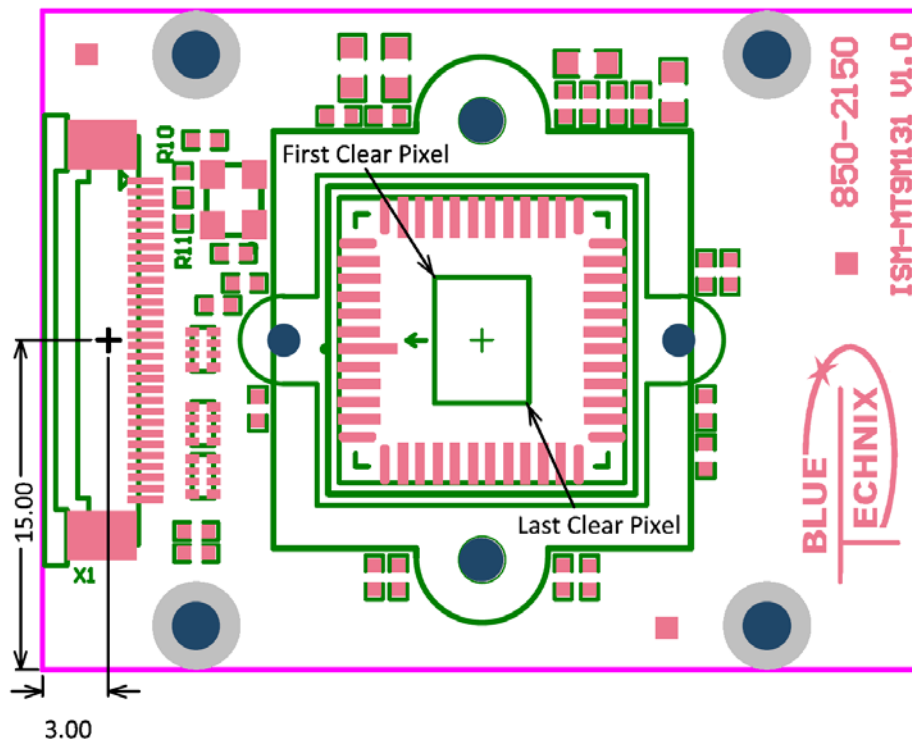
Figure 2-2: Top dimensions (connector position and sensor orientation)
