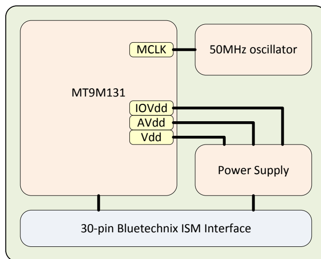
Figure 2-1: ISM-MT9M131 overview
