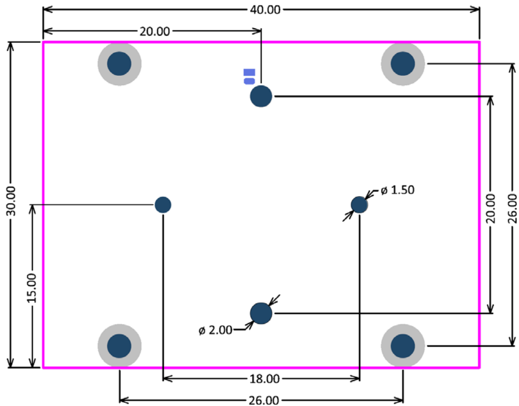
Figure 2-3: Bottom dimensions (mounting holes position)
