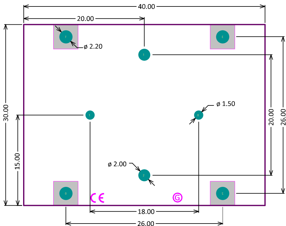
Figure 2-3: Bottom dimensions (mounting holes position)
