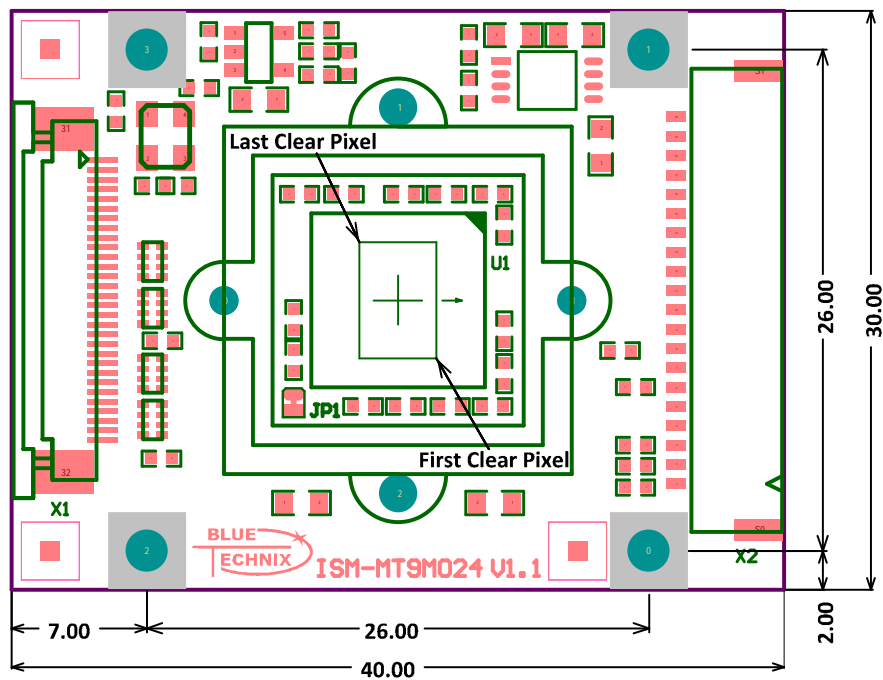
Figure 2-2: Top dimensions (connector position and sensor orientation)
