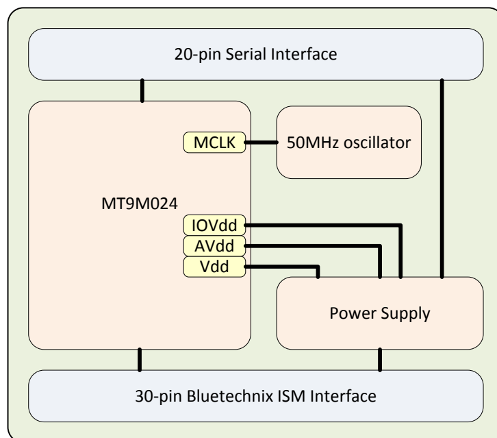
Figure 2-1: ISM-MT9M024 overview
