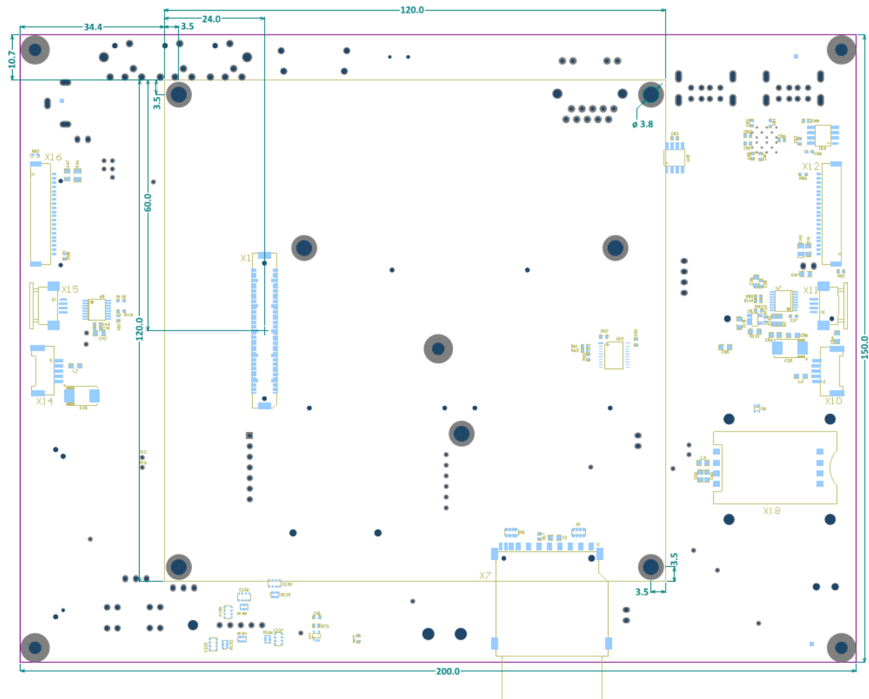
Figure 6-2 Mechanical outline bottom view
