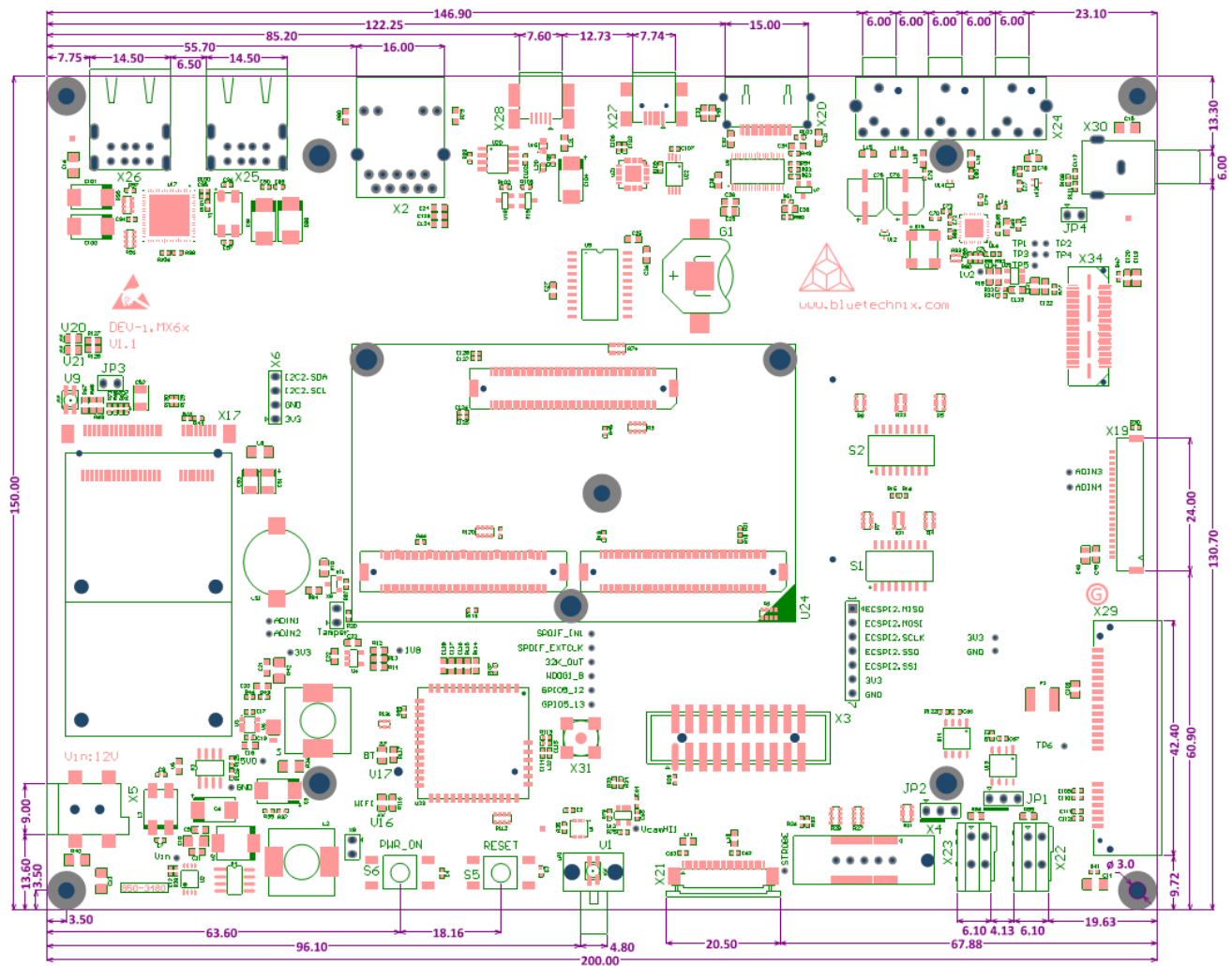
Figure 6-1 Mechanical outline top view
