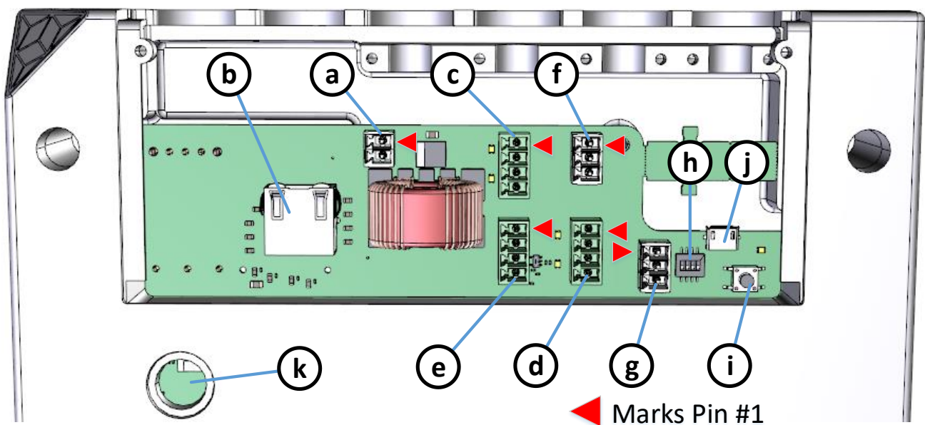
Figure 4-1: Argos3D-P33X connector location
