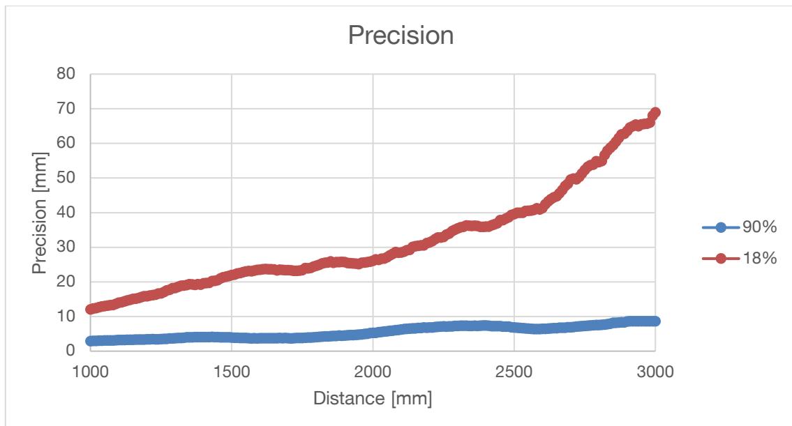
Figure 6-2: Typical precision
