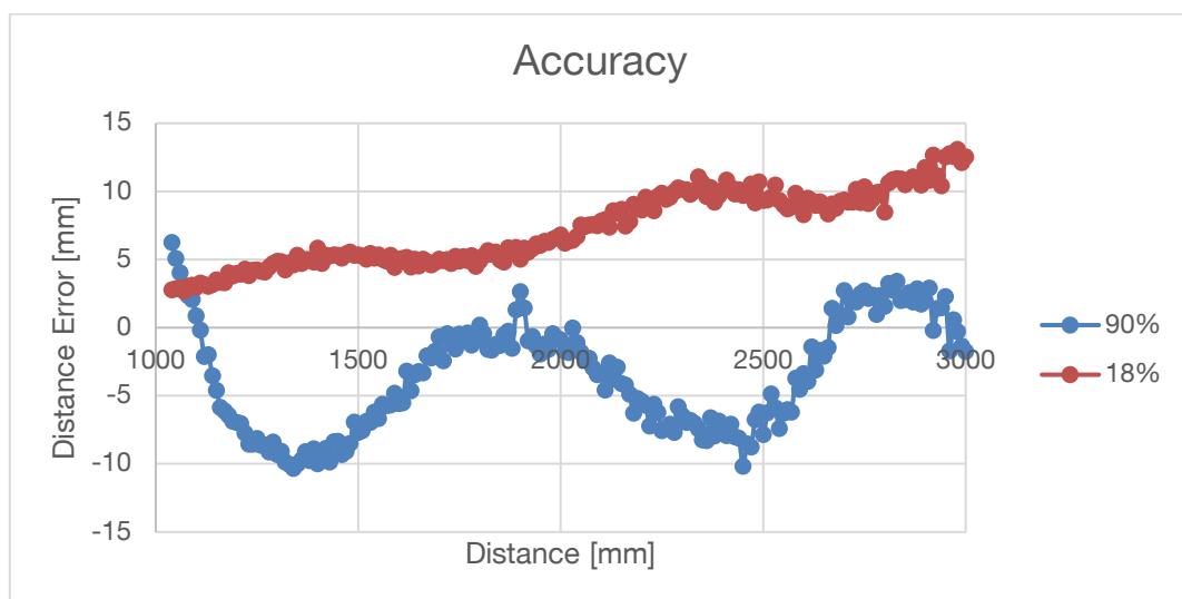
Figure 6-3: Typical accuracy
