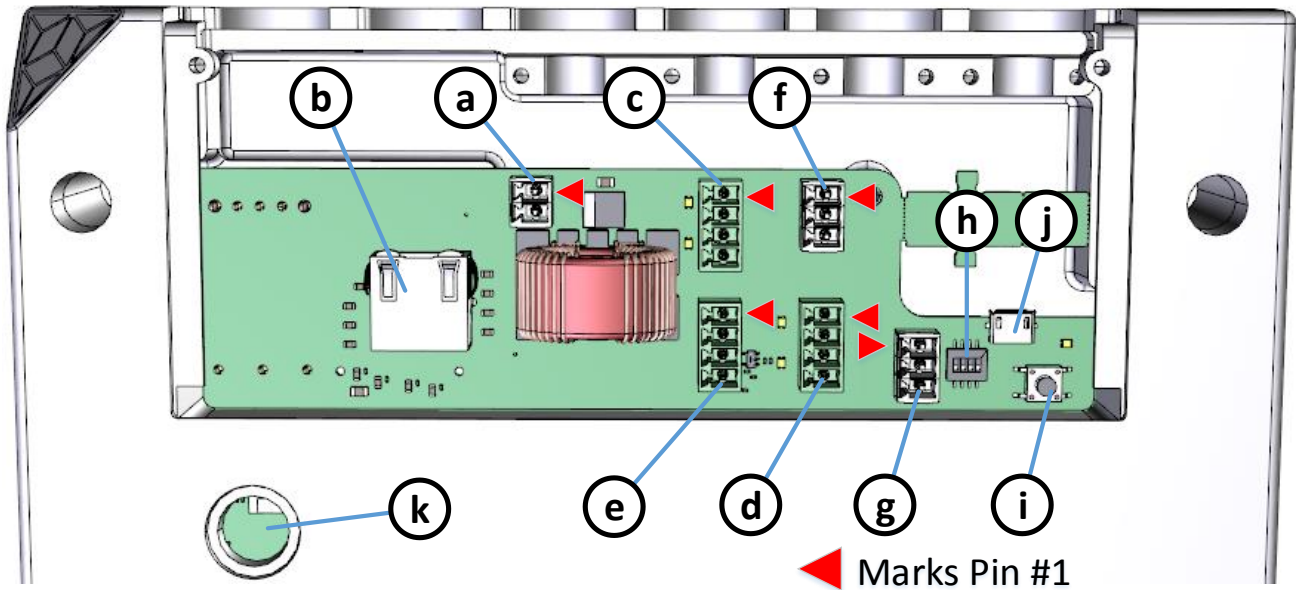
Figure 4-1: Argos3D-P32X connector location
