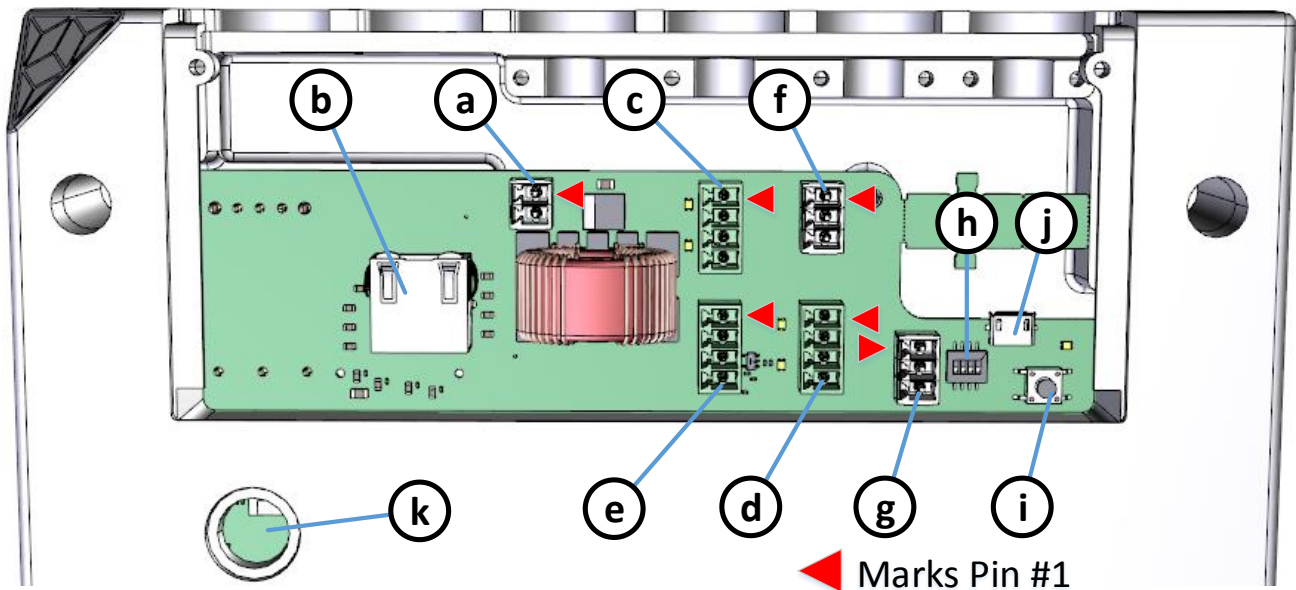
Figure 2-2: Argos3D-P32X connectors and interfaces
