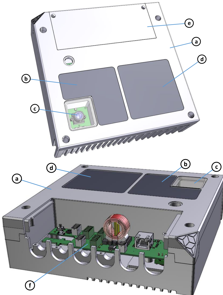
Figure 2-1 Argos3D-P32X components
