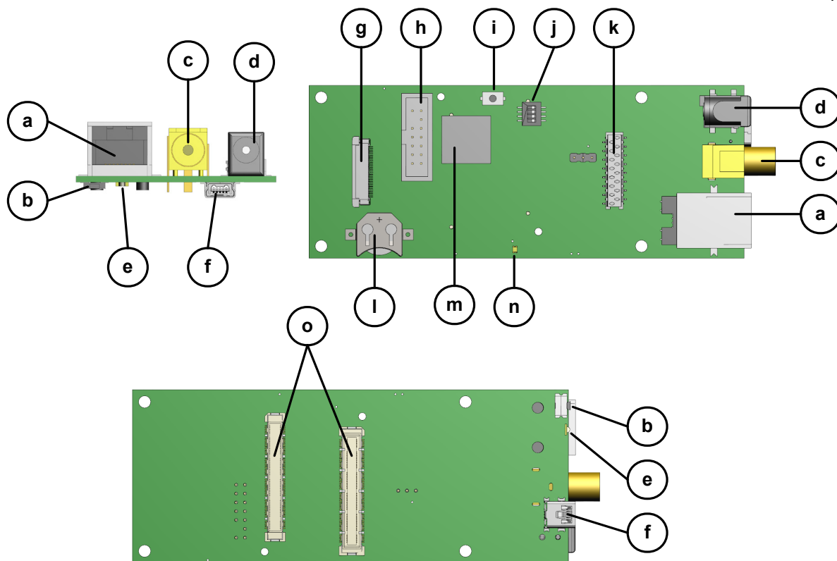
Figure 2.3: Argos2D – D10x connectors and interfaces
